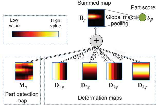
Figure 4. The deformation layer when deformation map is defined in (4). Part detection map and deformation maps are summed up with weights c_{n,p} for n = 1, 2, 3, 4 to obtain the summed map \mathbf{B}_p . Global max pooling is then performed on the summed map to obtain the score s_p for the p th part.
