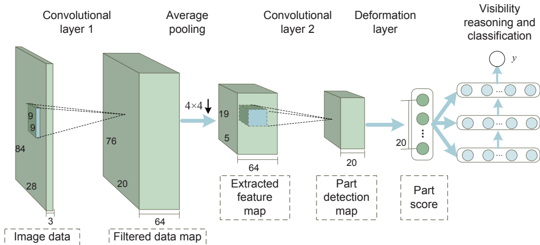
Figure 2. Overview of our deep model. Image data is convolved with 64 \ 9 \times 9 \times 3 filters and averagely pooled to obtain 64 feature maps. The feature maps are then processed by the second convolutional layer and the deformation layer to obtain 20 part scores. Finally the visibility reasoning model is used to estimate the detection label y .
