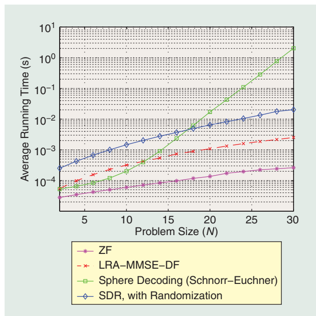
[FIG4] Complexity comparison of various MIMO detectors. SNR = 12 dB.
