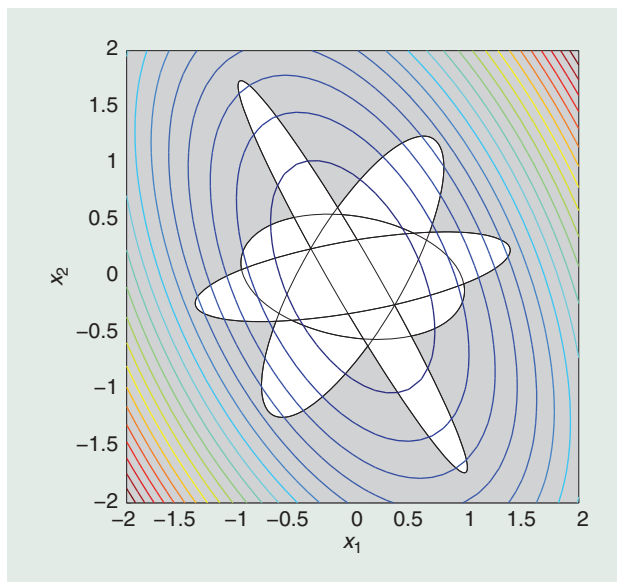
FIG1 A nonconvex QCQP in \mathbb{R}^2 : Colored lines represent the contour of the objective function, the gray area represents the feasible set, and the black lines represent the boundary of each constraint.
