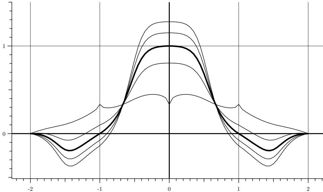
Figure 1. Family of basis functions that underly the computational procedure proposed by Salvado et al. 7 The most irregular curve corresponds to \lambda = \frac{1}{3} . The thick line corresponds to \lambda = 1 , the only case for which \phi_S is interpolant and continuously differentiable.
