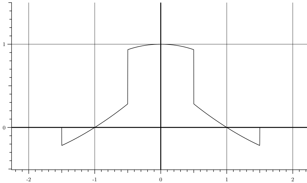
Figure 2. Proposed new basis function with order of approximation L = 2 . This order is identical to that of \varphi_S , but our proposed basis is shorter; yet, it has a larger capture range.
