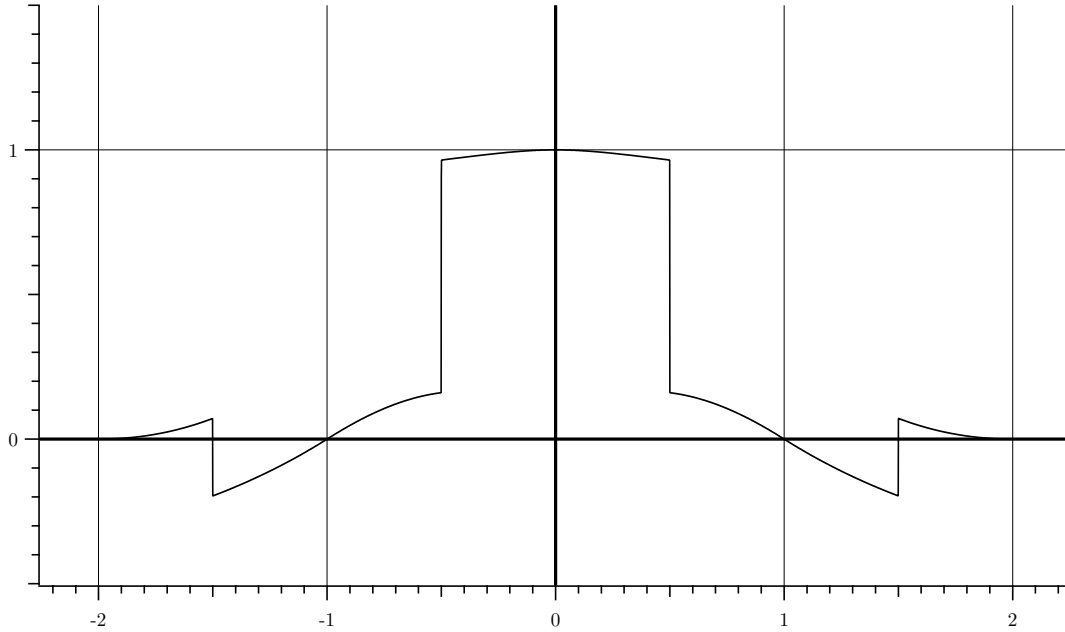
Figure 4. A basis function supported over [-2, 2] with the order of approximation L = 3 , which is one higher than that for \phi_S in Figure 1.
