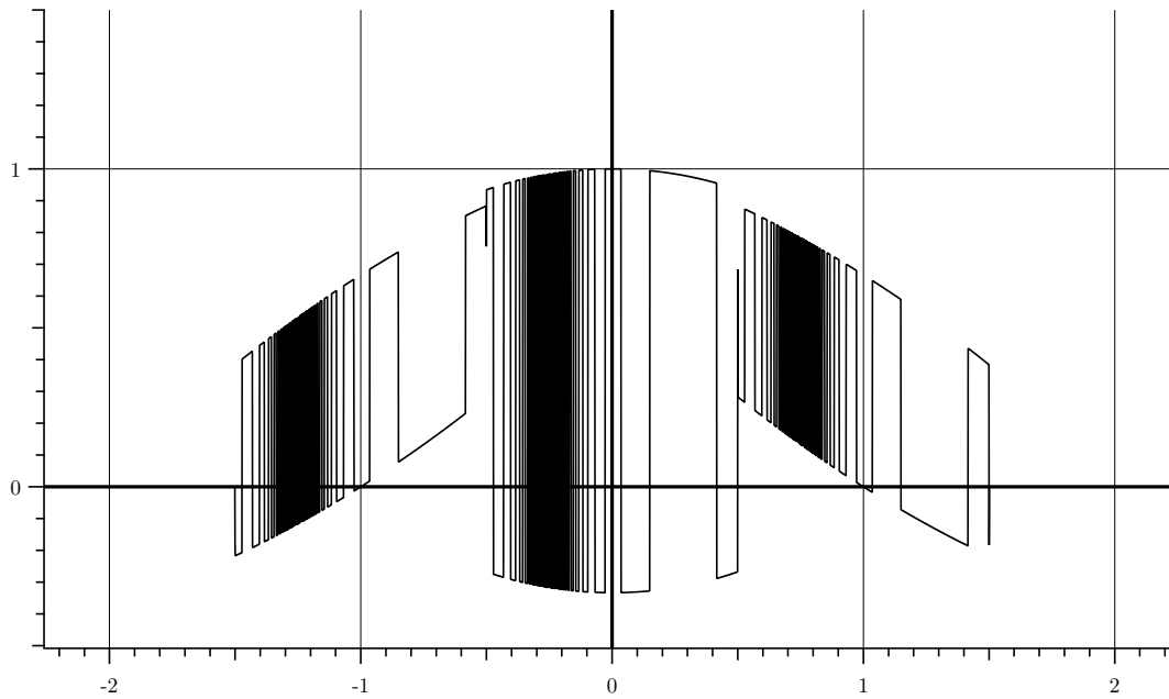
Figure 3. Another basis function supported over [-\frac{3}{2}, \frac{3}{2}] , with order of approximation L = 2 . This pathological basis has an infinite number of zero-crossings; it satisfies the partition of unity almost everywhere, but does not always offer pointwise convergence.
