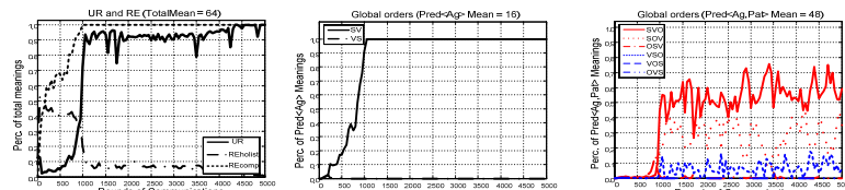
Figure 3. Coevolution of compositionality and regularity. RC=0.6. CT=0.75.
